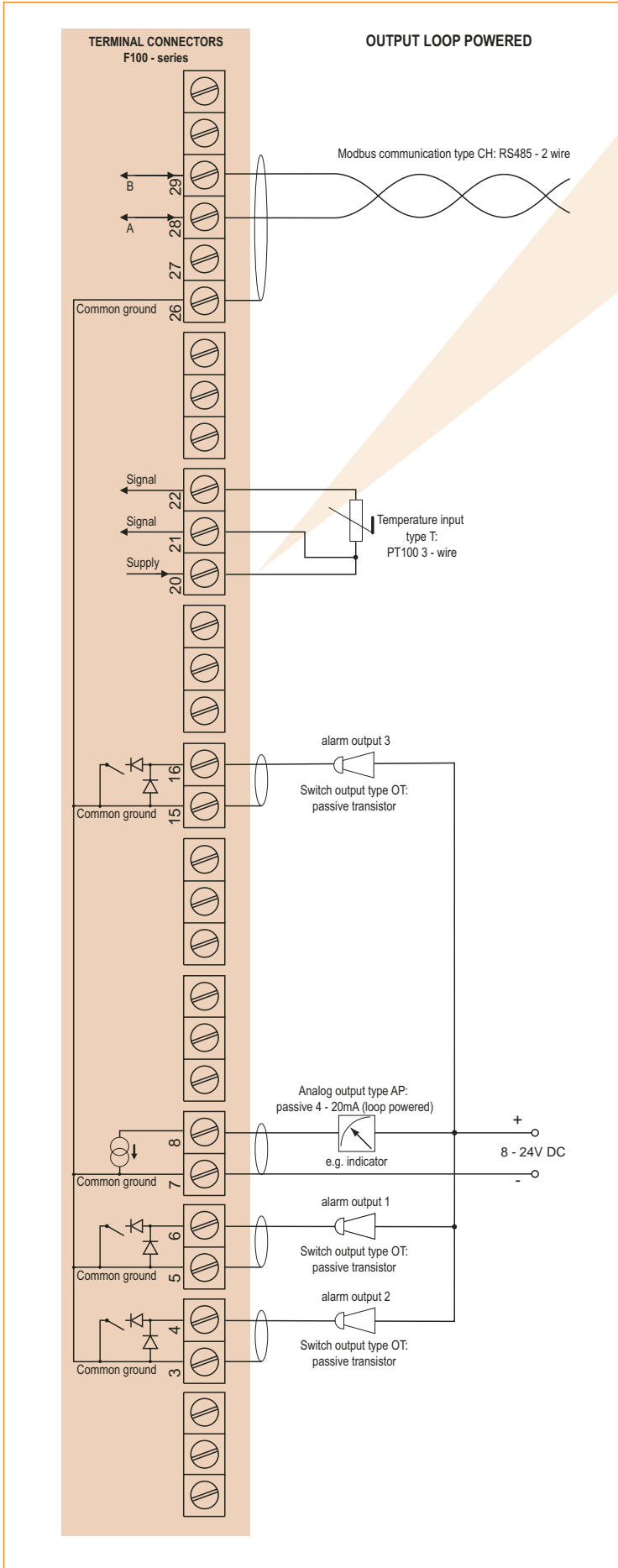
Typical wiring diagram F143-T-AP-CH-OT
