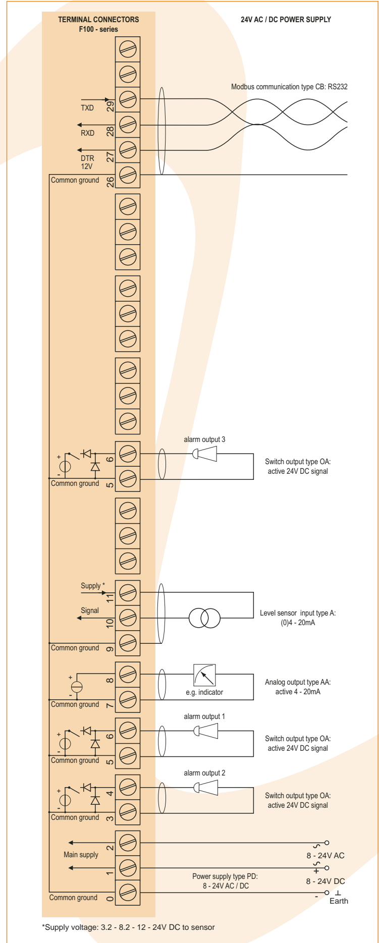
Typical wiring diagram F170-A-AP-CH-OT
