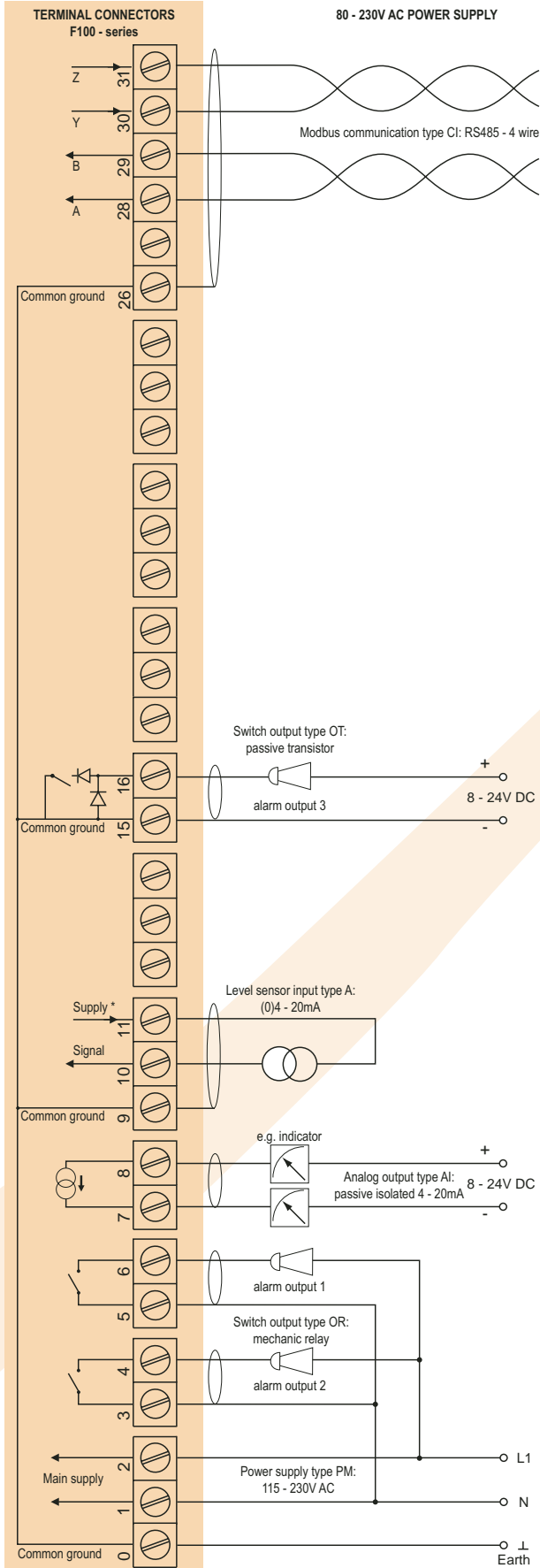
Typical wiring diagram F170-P-AP-CB-OS-PD
