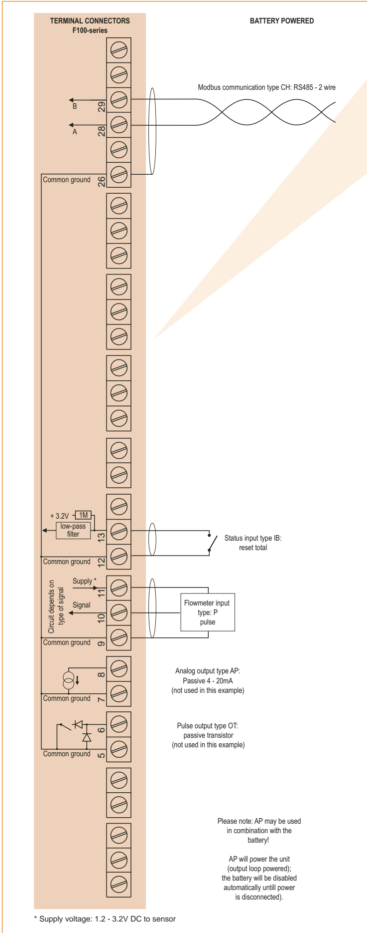
Typical wiring diagram F112-P-(AP)-CH-IB-PB-(OT)
