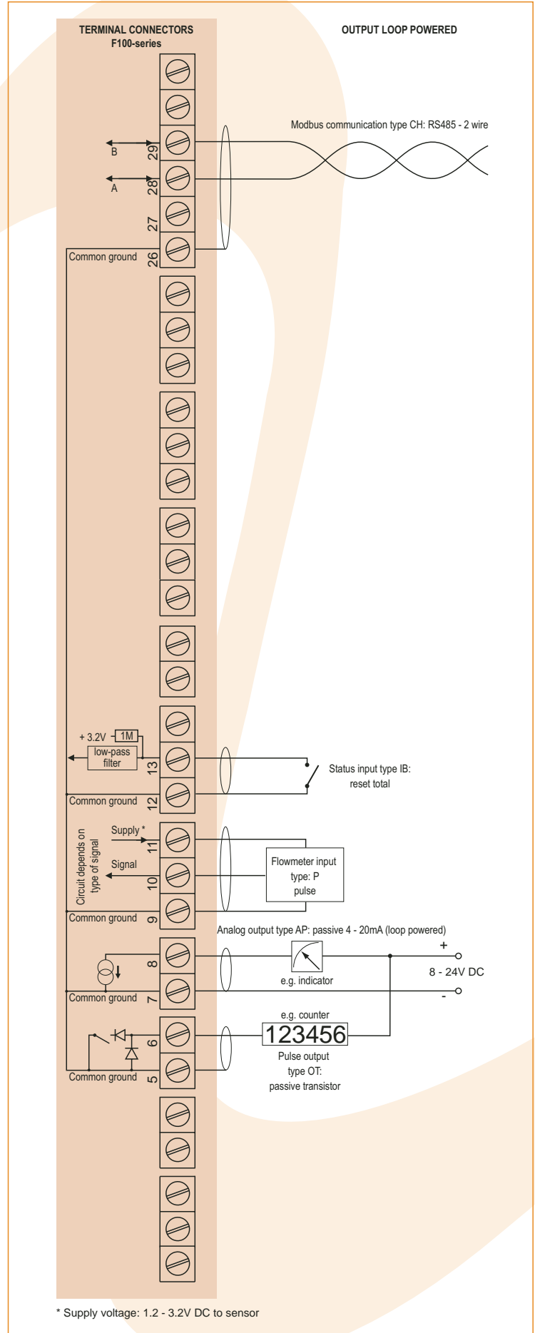
Typical wiring diagram F112-P-AP-CH-IB-OT
