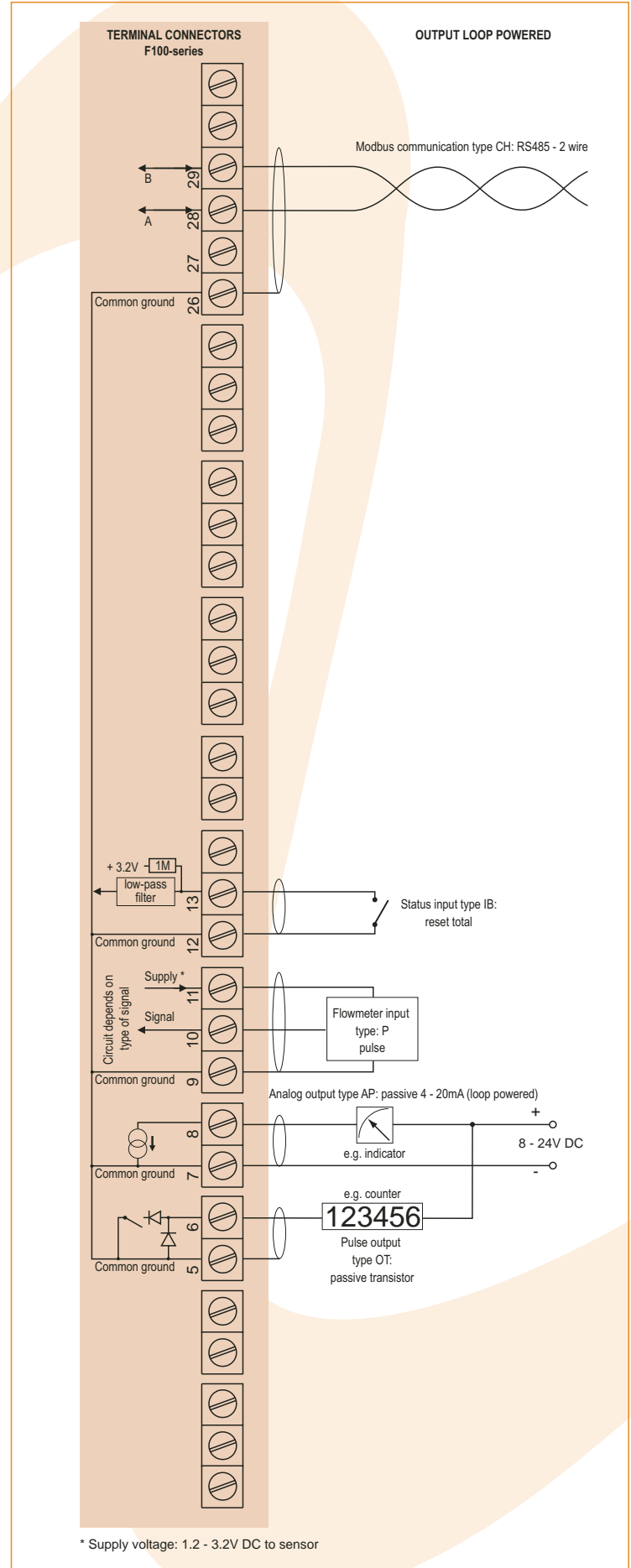
Typical wiring diagram F110-P-AP-CH-IB-OT
