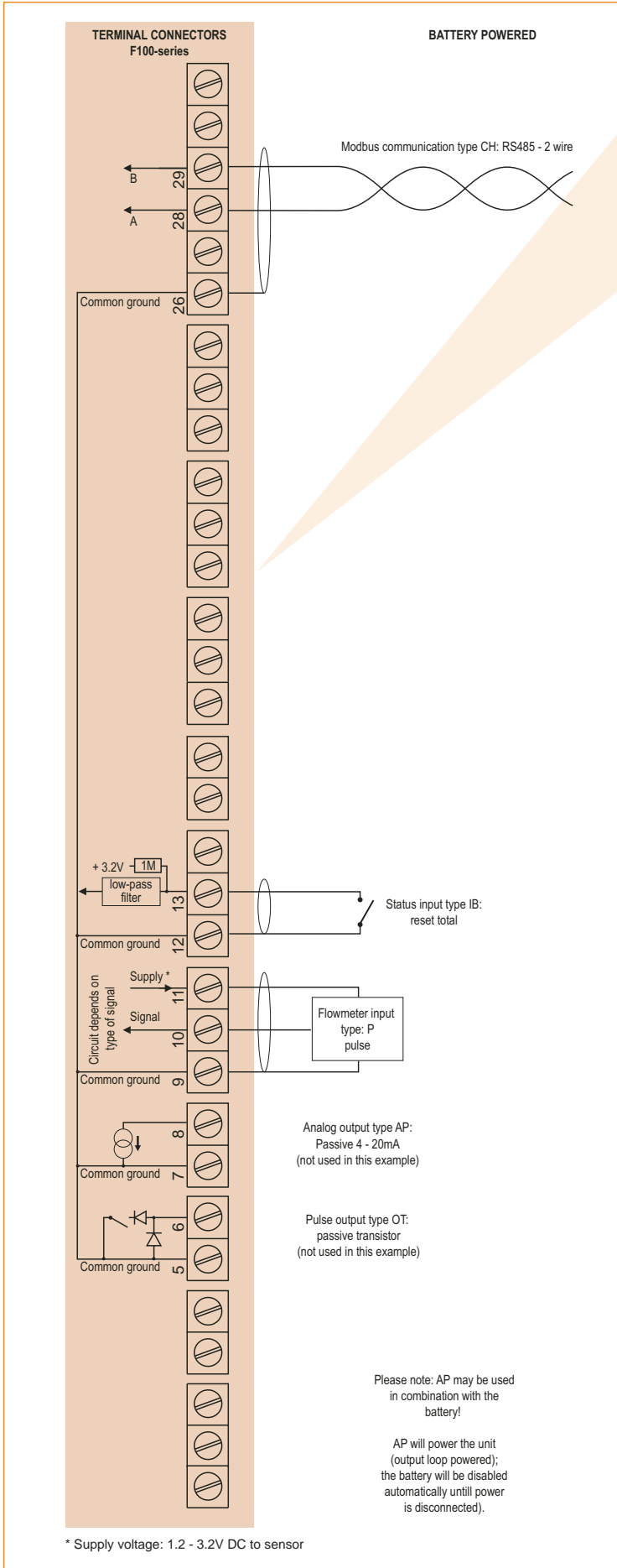
Typical wiring diagram F110-P-(AP)-CH-IB-PB-OT
