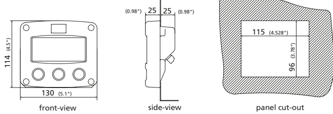
ENCLOSURE HC (STANDARD) ABS PANEL MOUNT ENCLOSURE
