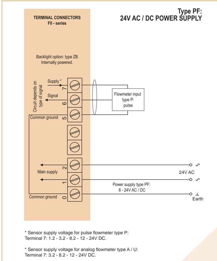
Typical wiring diagram F010-P-PF-ZB
