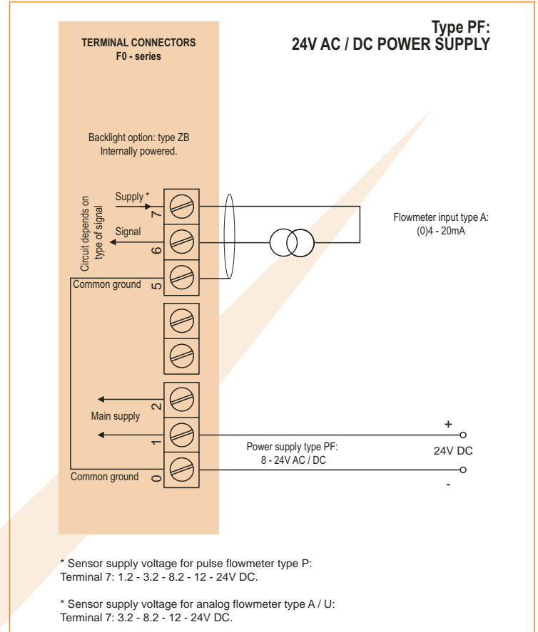
Typical wiring diagram F010-A-PF-ZB
