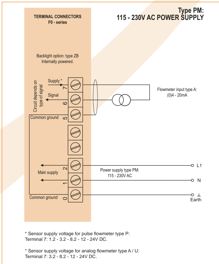
Typical wiring diagram F010-A-PM-ZB
