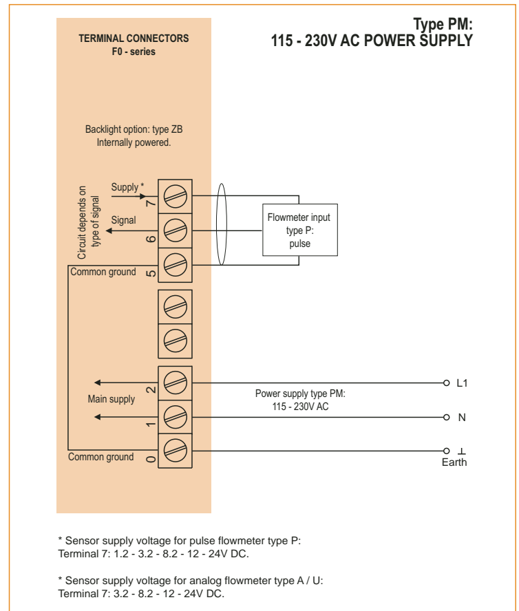
Typical wiring diagram F010-P-PM-ZB
