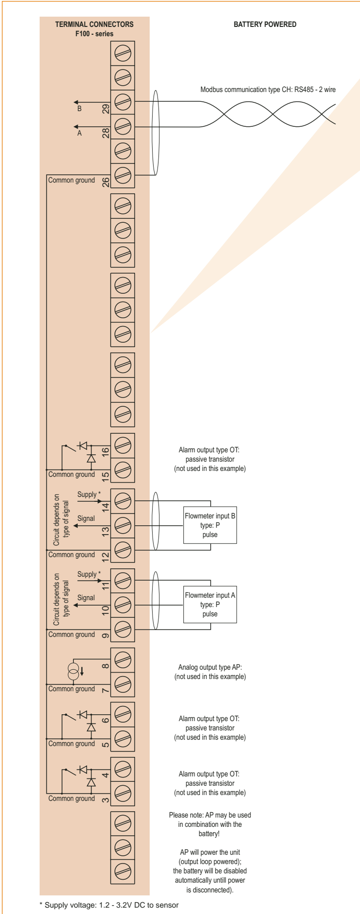
Typical wiring diagram F114-P-(AP)-CH-PB-(OT)
