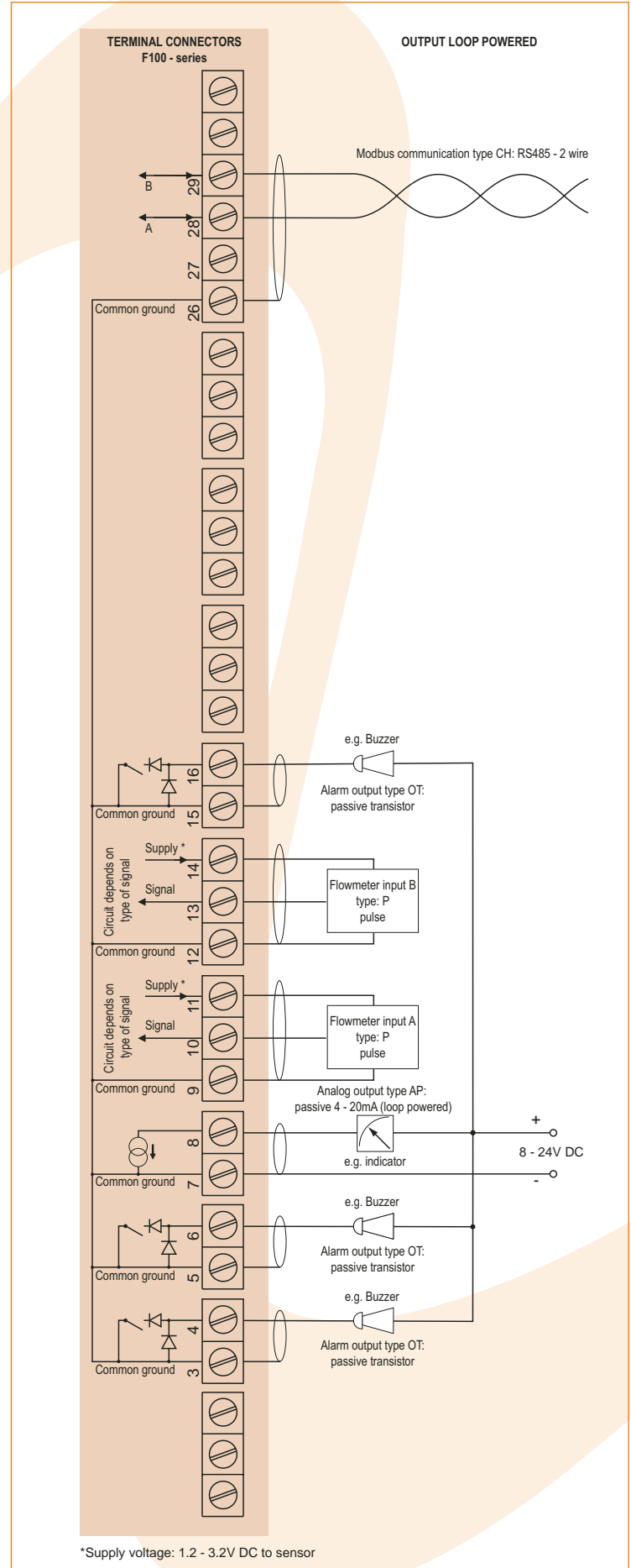
Typical wiring diagram F114-P-AP-CH-OT
