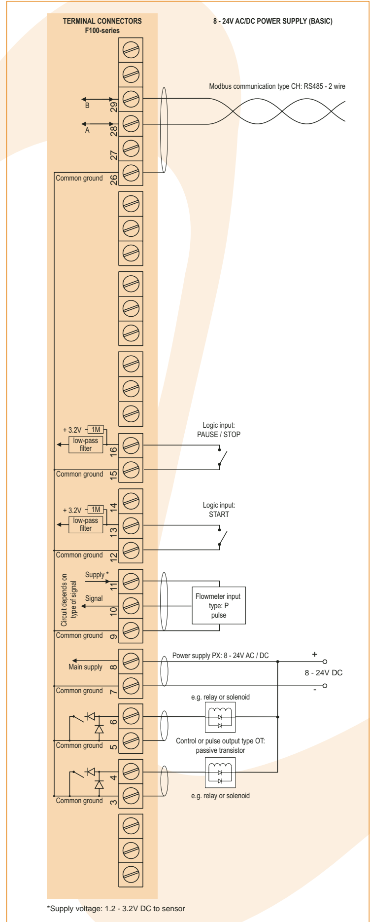
Typical wiring diagram F130-P-CH-PX-OT
