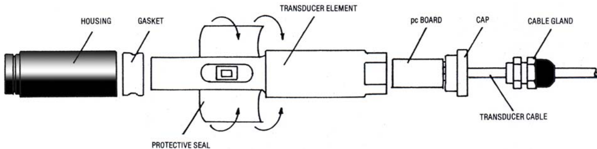
Double Cantilever Beam Construction
