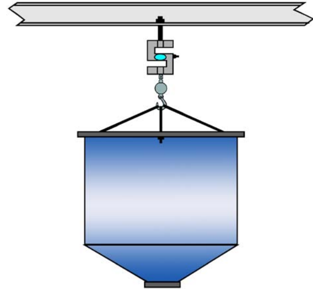
Simple, single U3SB tension mount system
