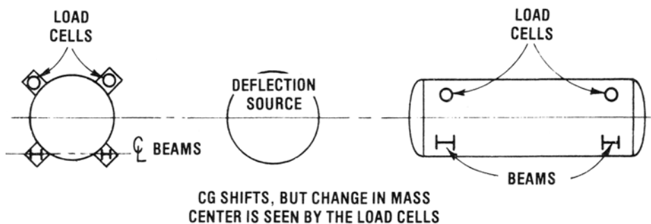
Correct mounting arrangement for partially supported vessels experiencing deflection duress
