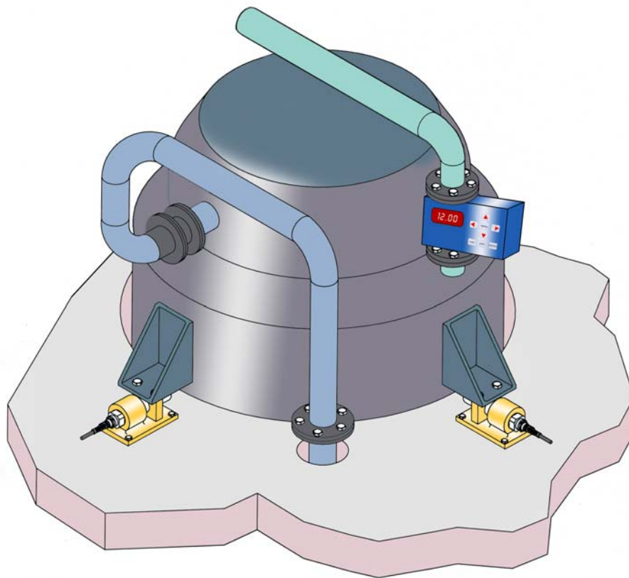
Flowmeter based measurement system with redundant weigh module backup
