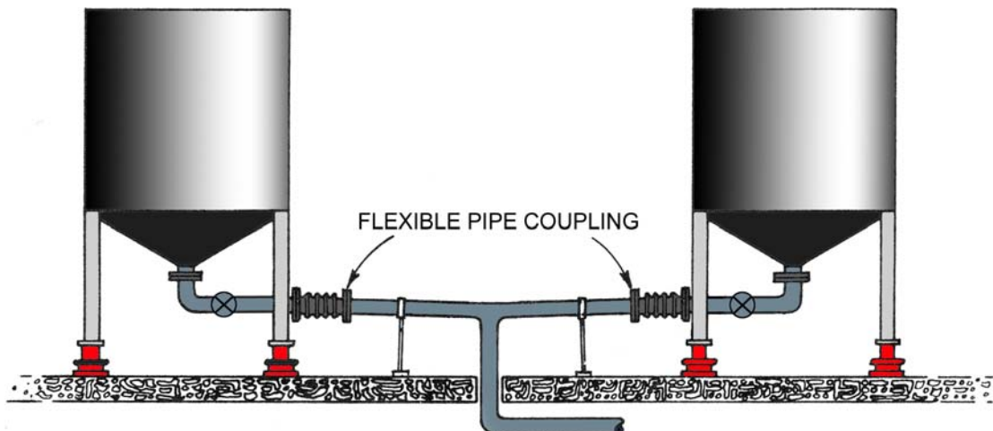
Install flexible pipe coupling for each tank sharing the common drain
