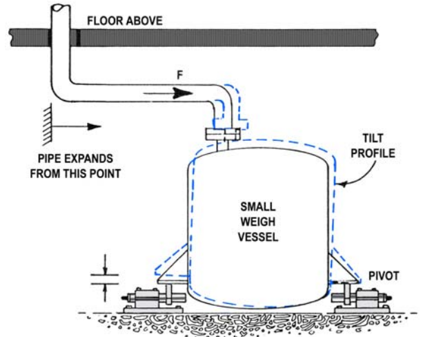
Piping expands from fixed support to vessel attachment as hot fluid passes through.
