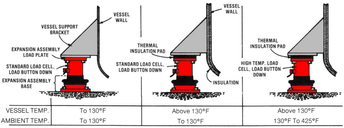
Thermal expansion and contraction accessories
