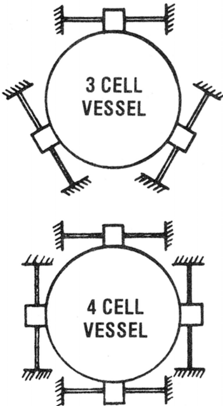
Lateral restraints on three and four cell vessels
