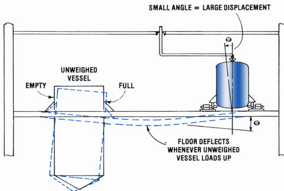
Incorrect piping arrangement for floor deflection. Support pipe from same floor weigh vessel rests upon
