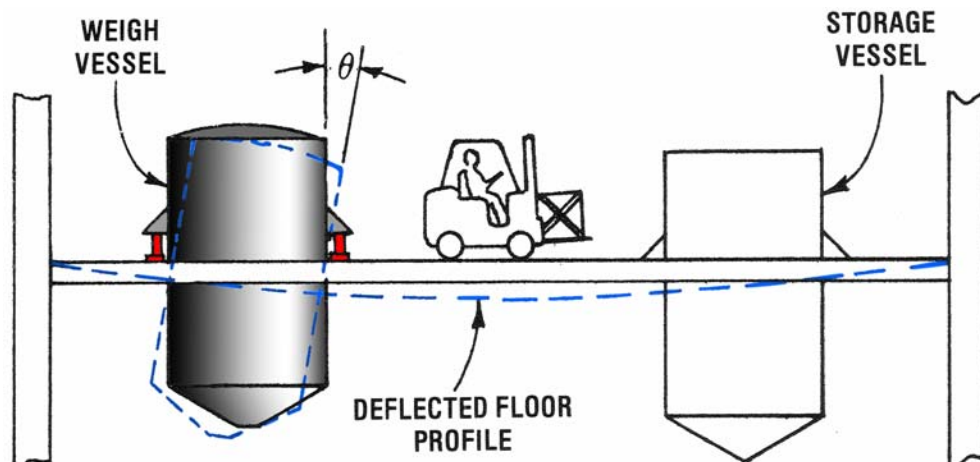
Vessel Tilts with Increasing Load
