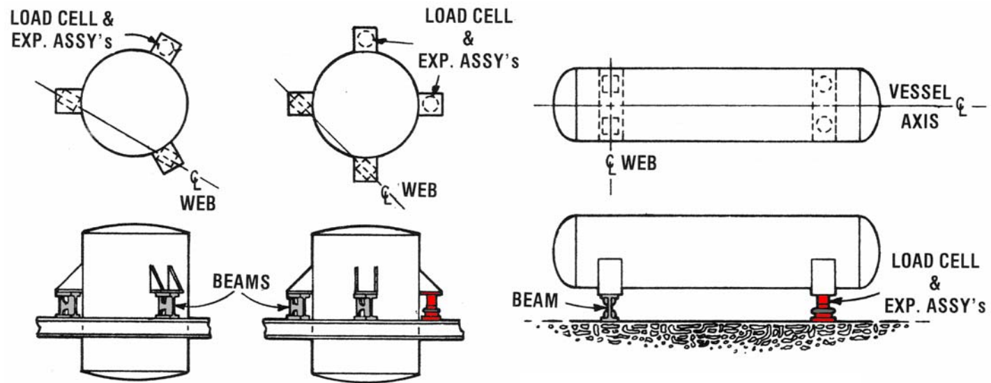
APPLICATIONS: Align beam webs so vessel can pivot with load cell deflection
