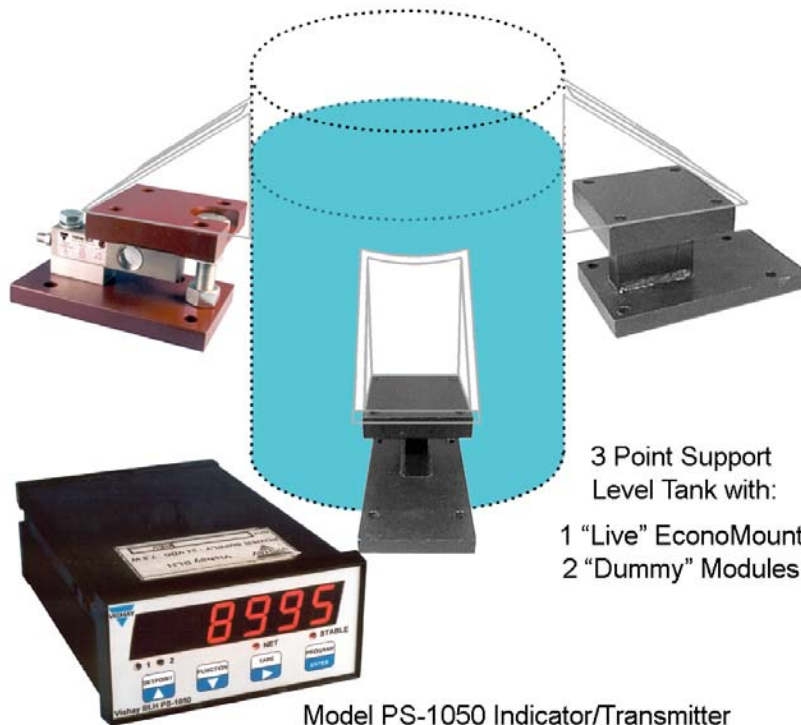
Simple level system with single weigh module support
