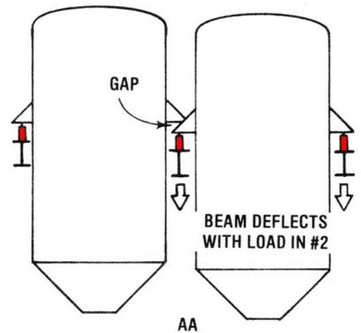
Use three-point supports to eliminate possibility of gapping
