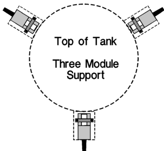
Weigh module mounting footprint
