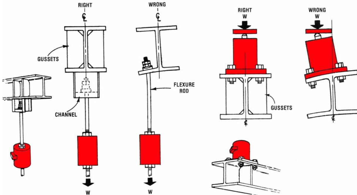
Correct and incorrect methods of load cell alignment
