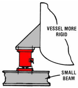
Fixed mounting plates: standard mounting kit when vessel and support structure are both at ambient temperature
