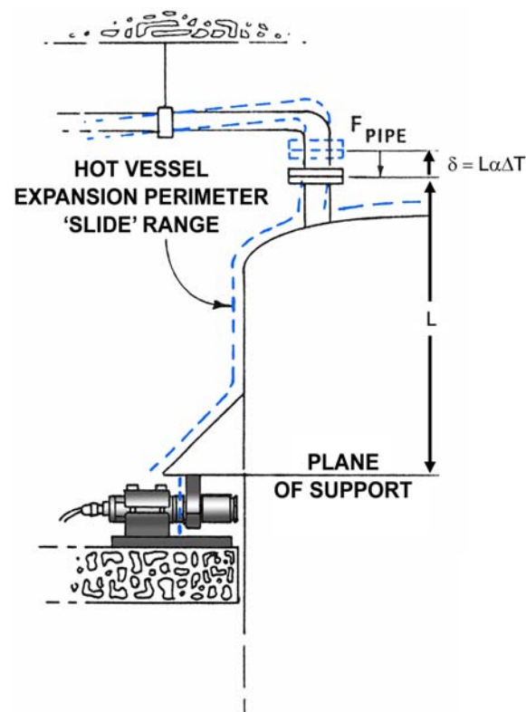
Vessel restriction due to thermal expansion
