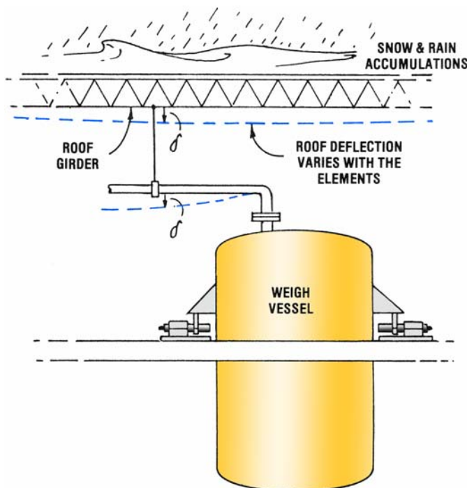
Pipe supports, especially the first supports away from vessel, deflect under random influences, generating vertical pipe forces on weigh vessel.
