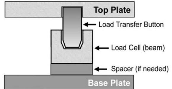
Typical Load Cell Weigh Module Construction
