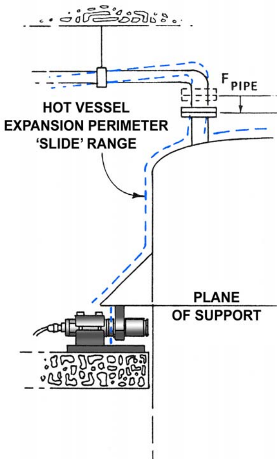
Heated vessel thermal expansion and contraction
