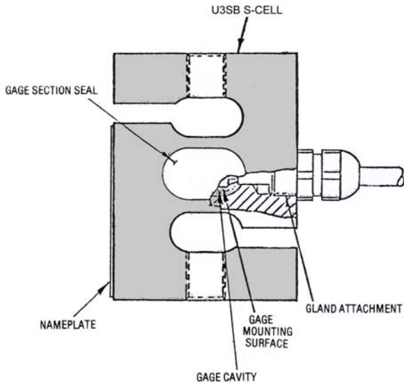
S-Cell Construction
