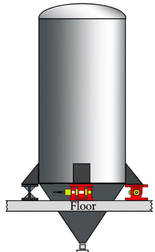
Lower accuracy storage silo partially supported by KDH Weigh Modules
