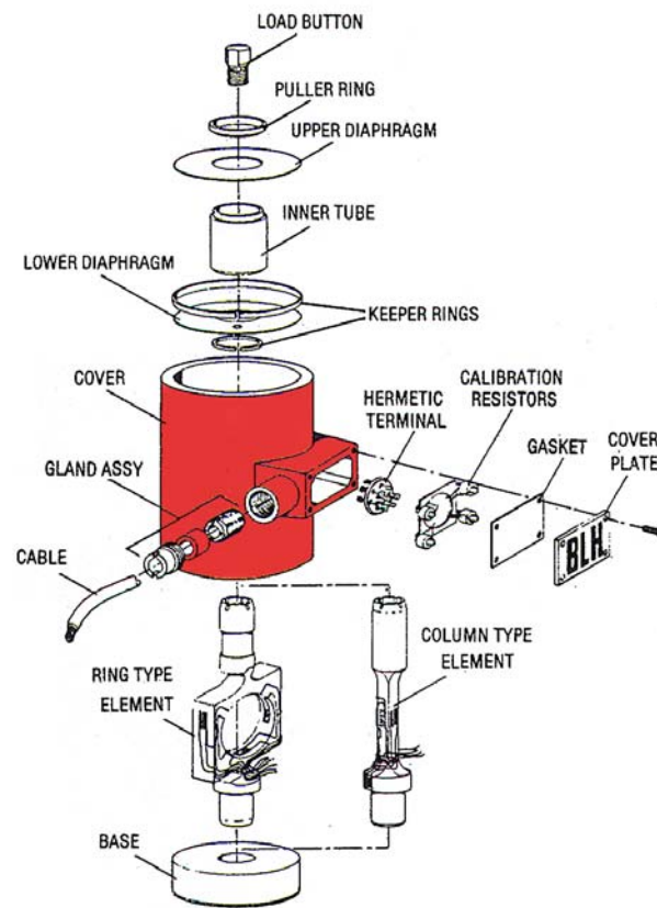
Canister Cell Construction
