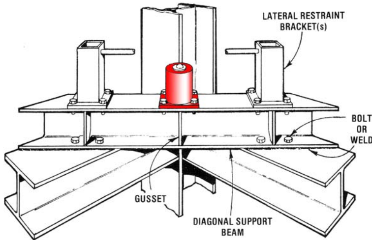
Load cell mounting - preferred arrangement
