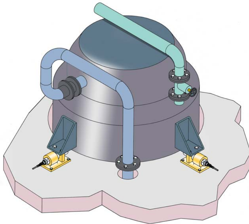
Precision compression system with KIS Weigh Modules mounted on concrete floor
