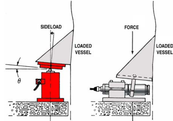
Loaded vessel - wall deflection
