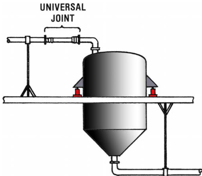
RECOMMENDED PIPE SUPPORT ARRANGEMENT
