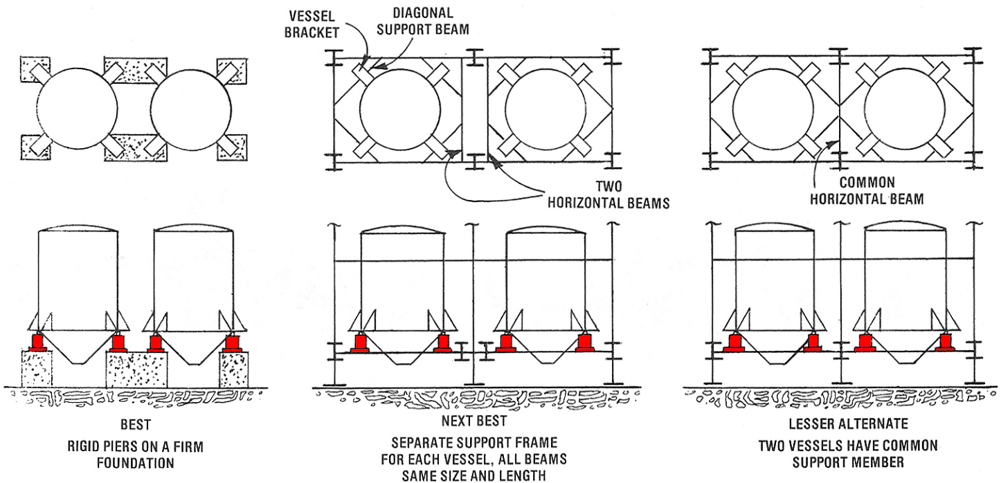
Adjacent vessel mounting arrangements
