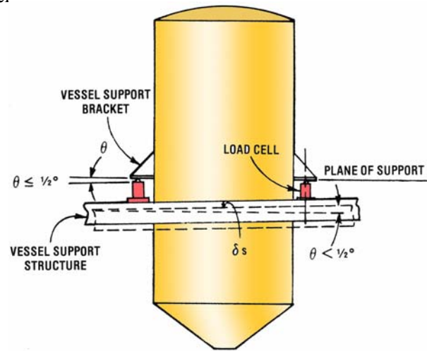
Support Bracket Tilt
