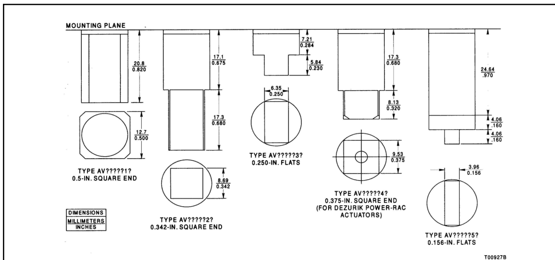
Figure 8. Drive Shaft Variations
