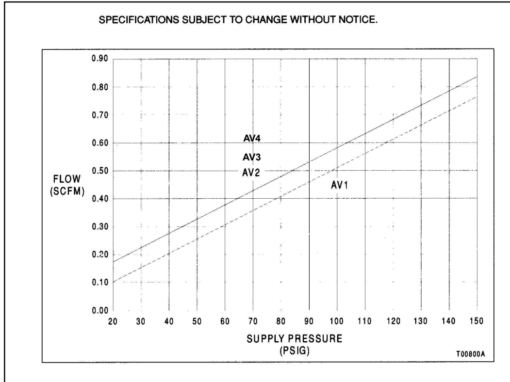
Figure 1. Air Consumption (at Null)
