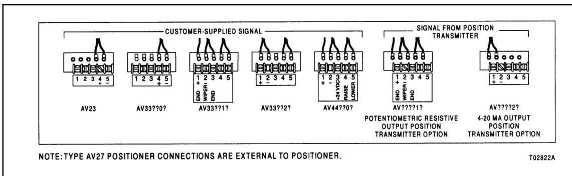
Figure 9. Electrical Connections
