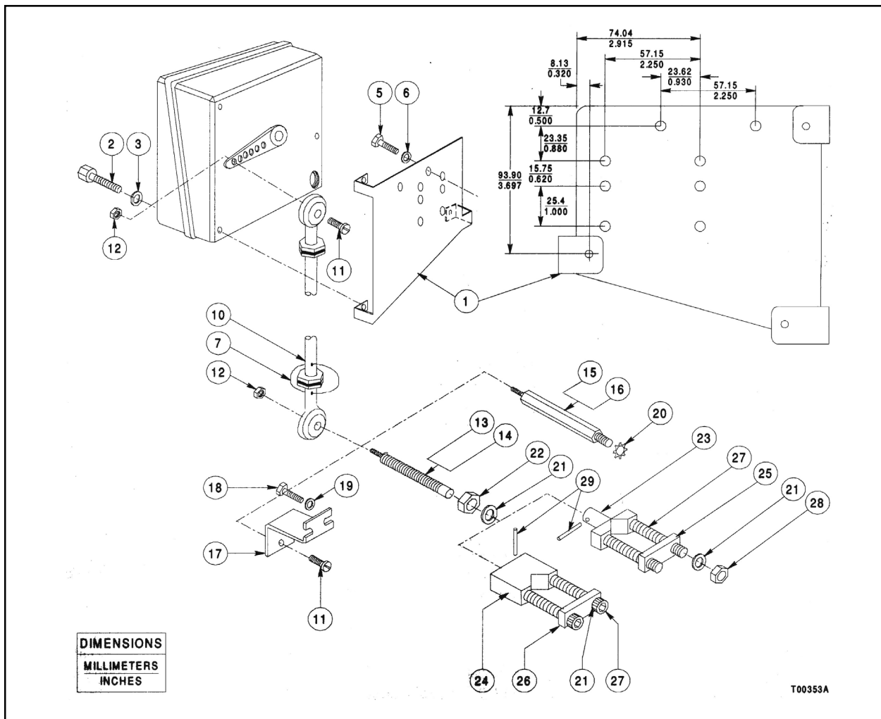
Figure 10. Mounting Kits
