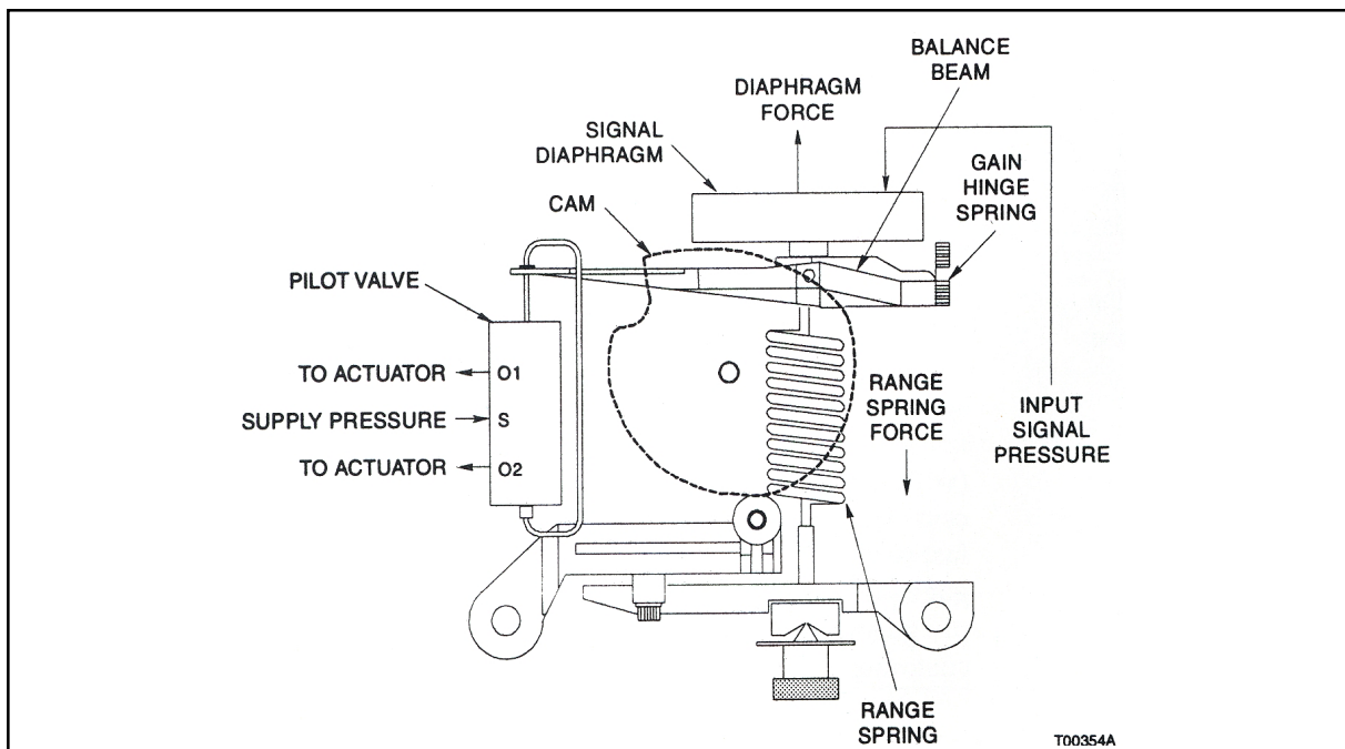
Figure 4. Operation Diagram
