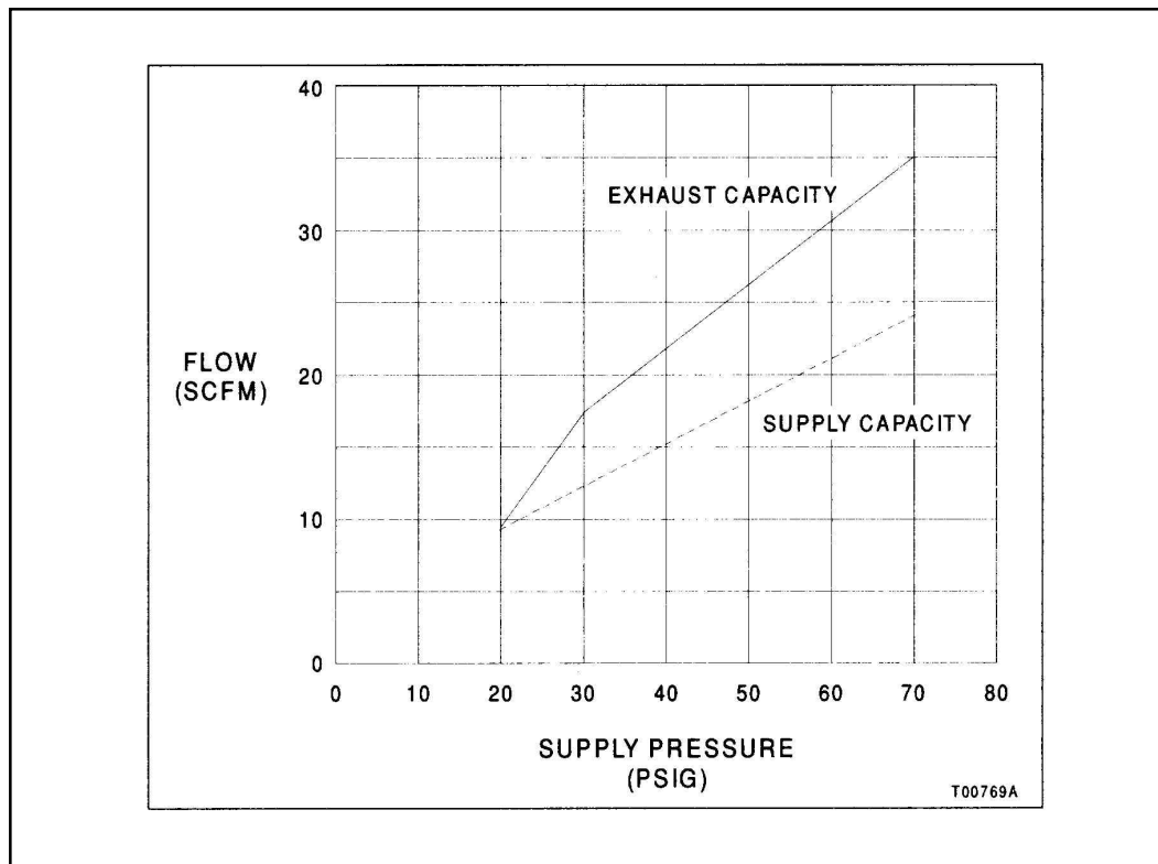
Figure 2. Capacity (Exhaust to Atmosphere)
