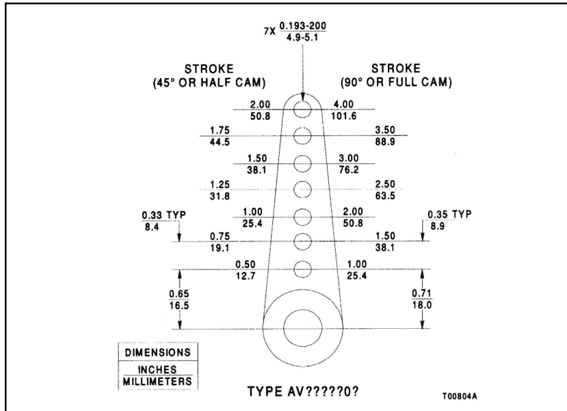
Figure 7. Drive Arm Connections
