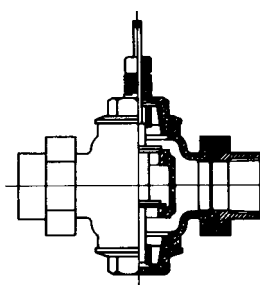
Style FA Double Seated Semi-Balanced Rev. Acting: 3/4" - 1 1/2" Bz body; Bz unions; Trim Bz or Monel 2" - 4" Cl or Bz body; Flgd; Trim Bz, SS or Monel Dir. Acting: 2 1/2" - 4" Cl or Bz body; Flgd; Trim Bz or SS
