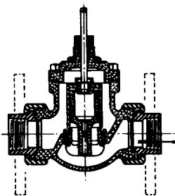
Style MA Single Seated Fully Balanced Direct Acting only Sizes 3/4" - 1 1/2" Bronze or Steel, 2" Bronze, Cast Iron or Steel SS Trim
