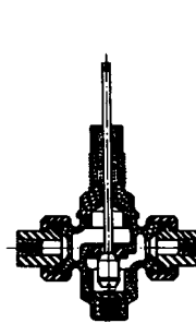
Style WA, Union Ends Unbalanced sizes 1/2" - 1 1/2" Bronze Body SS Trim
