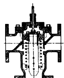
Style WD Balanced Sizes 2" - 2 1/2" Bronze Body, Flgd Bronze Trim
