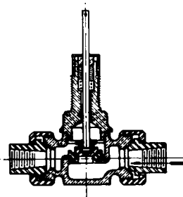
Style A, Union Ends Single seated Unbalanced Direct acting sizes 1/4" - 1" Reverse acting sizes 1/4" - 1" Bronze body SS trim
