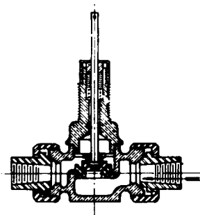
Style A, Union Fads. Single Seated Unbalanced Direct 8c Rev. Acting Sizes 1/4" - 1 1/2" Bronze SS Trim
